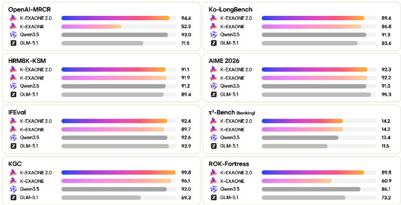
자료: LG Research, Huggingface, 대신증권 Research Center
